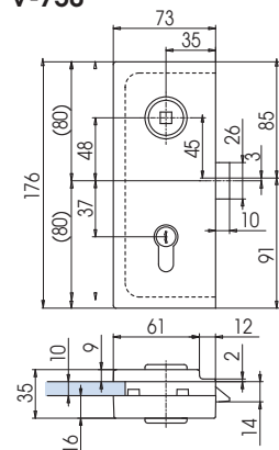
V-750 PZ-R destra/right
