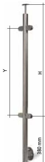
R = Reggicorrimano snodato - Pivotable handrail support
