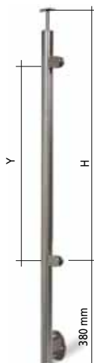
R = Reggicorrimano snodato - Pivotable handrail support
