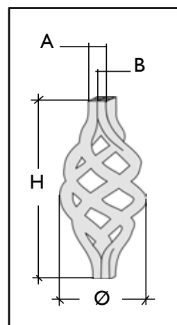
Art. 1163/9 \varnothing 70 mm B = \varnothing 6 mm
