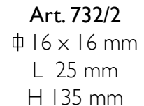
Art. 732/2 Φ 16 x 16 mm L 25 mm H 135 mm Foro-Hole Φ 16 mm
