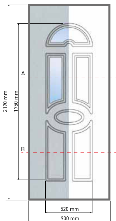
▼ Vista esterna | External view
