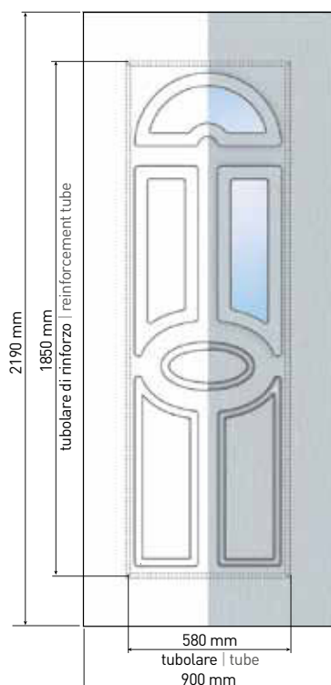
▼ Vista interna | Internal view
